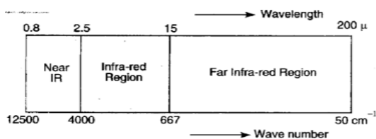
Fig. 3.1. Infra-red region.
