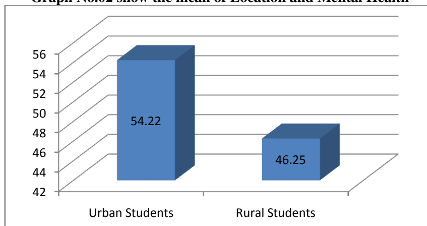
Graph No.02 show the mean of Location and Mental Health
